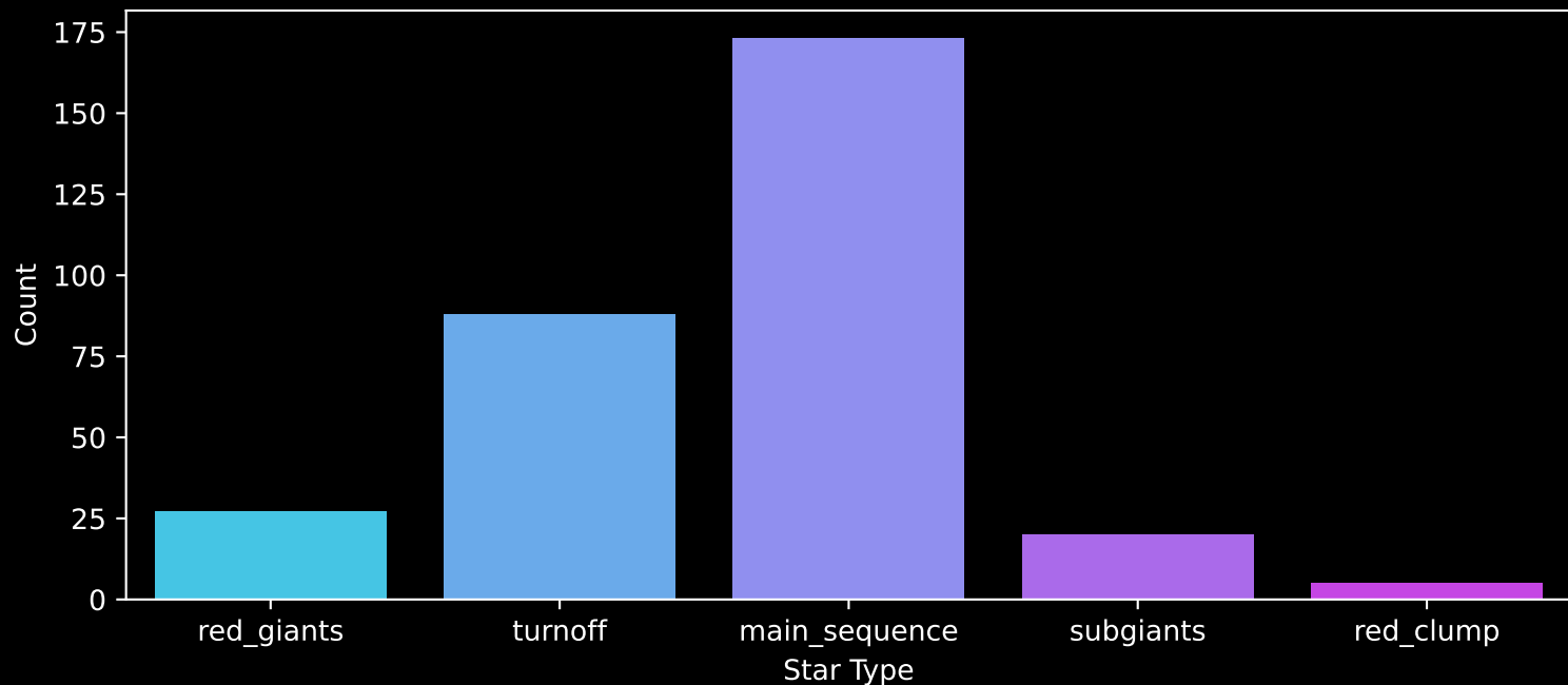
GALAH DR4 Field: [419] Count plot of Star Type
