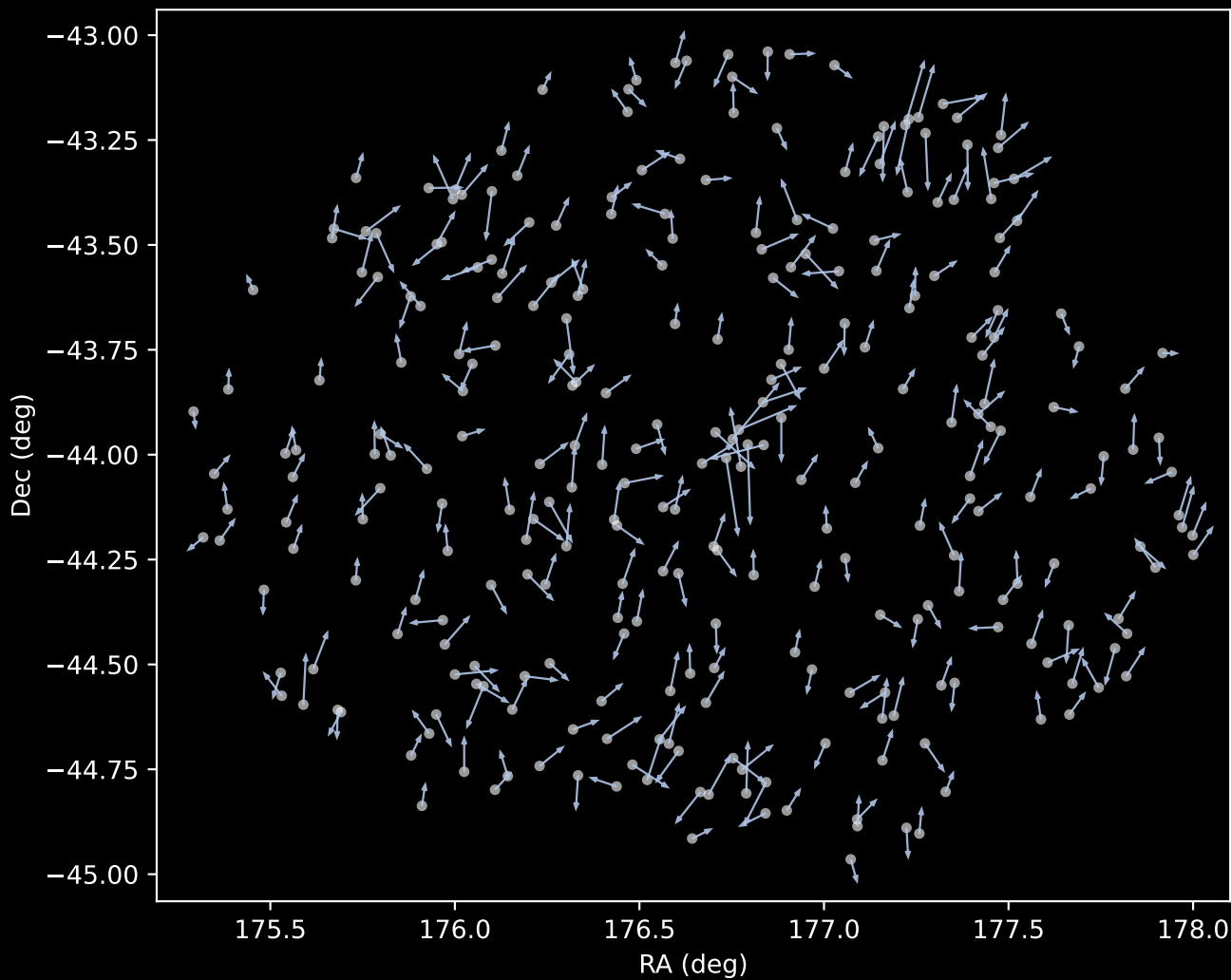
GALAH DR4 Cluster 1 Proper Motion Vectors (n=287)
