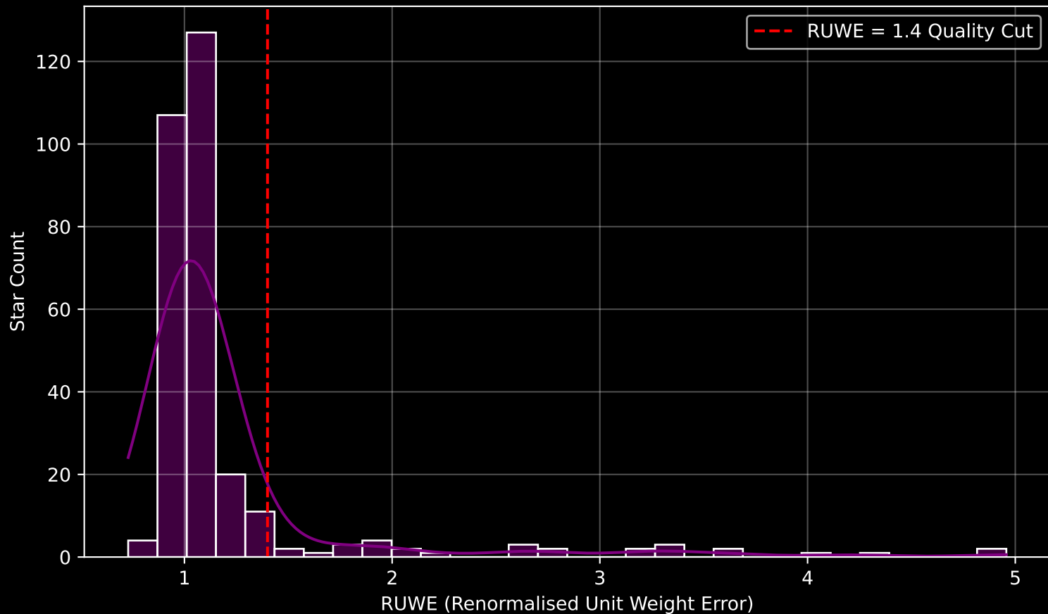
GALAH DR4 Field [419] RUWE Distribution (n= 298)
